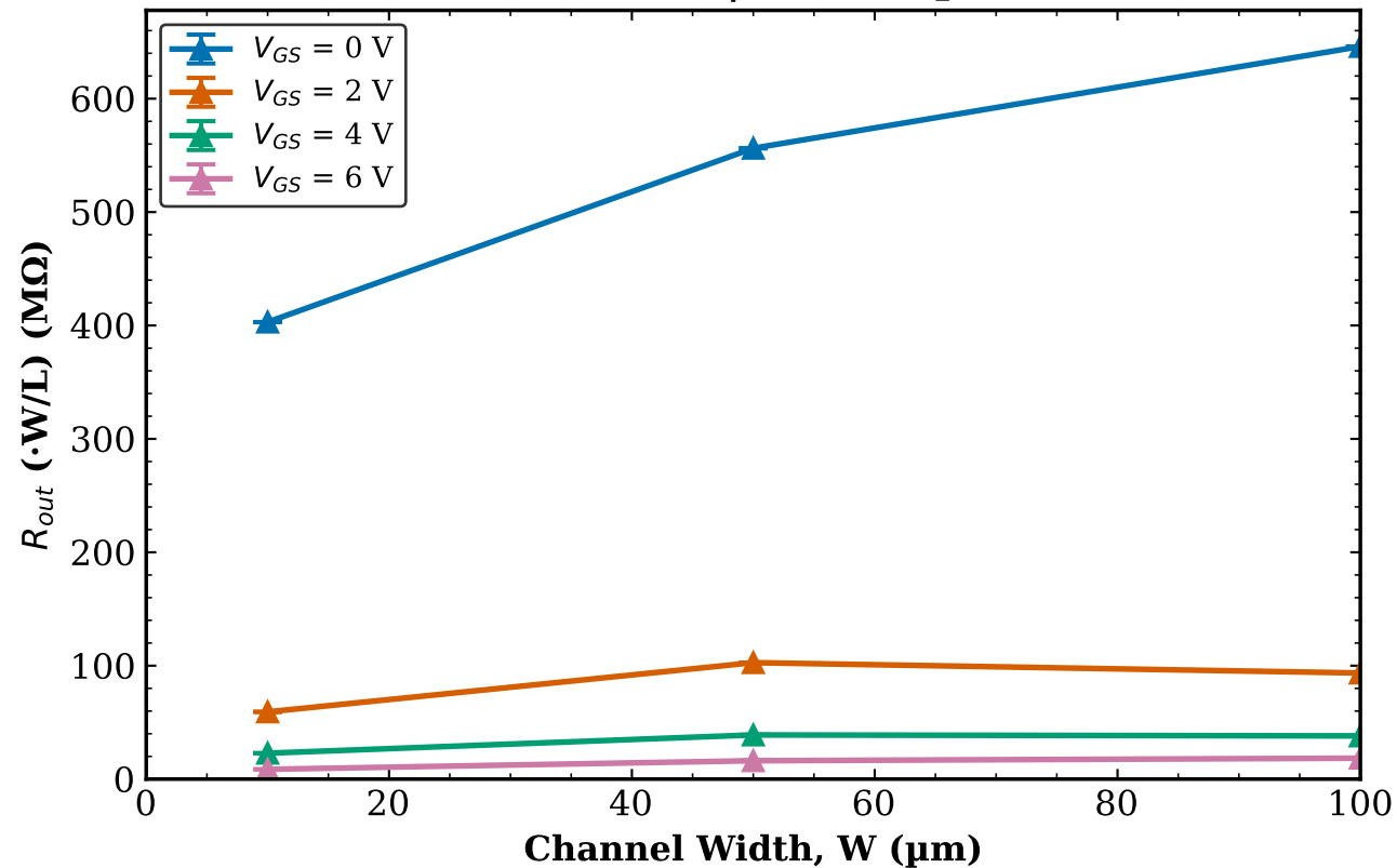
TFT1 Transistor 2 R_{out} vs W | L = 40\text{ }\mu\text{m}
